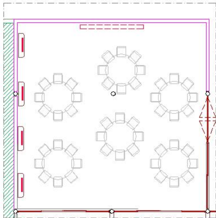
PLANTA BAIXA - COFFEE SHOP
